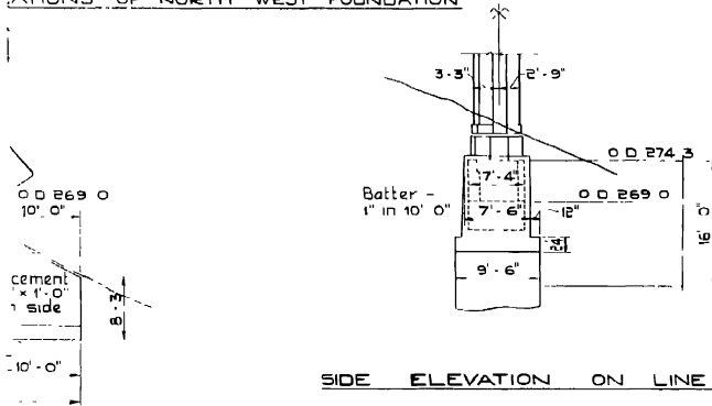
ELEVATIONS OF NORTH WEST FOUNDATION
